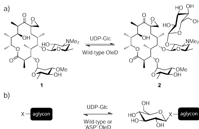
Scheme 1. a) Natural reaction catalyzed by WT OleD. b) General reaction for probing aglycon promiscuity in vitro against a panel of 137 library members; X = OH, SH, NH 2 , or NHR.
