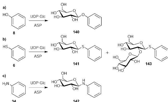
Scheme 2. Products isolated from large scale enzymatic reactions of ASP OleD with a) phenol ( 8 ), b) thiophenol ( 6 ), and c) aniline ( 34 ).
