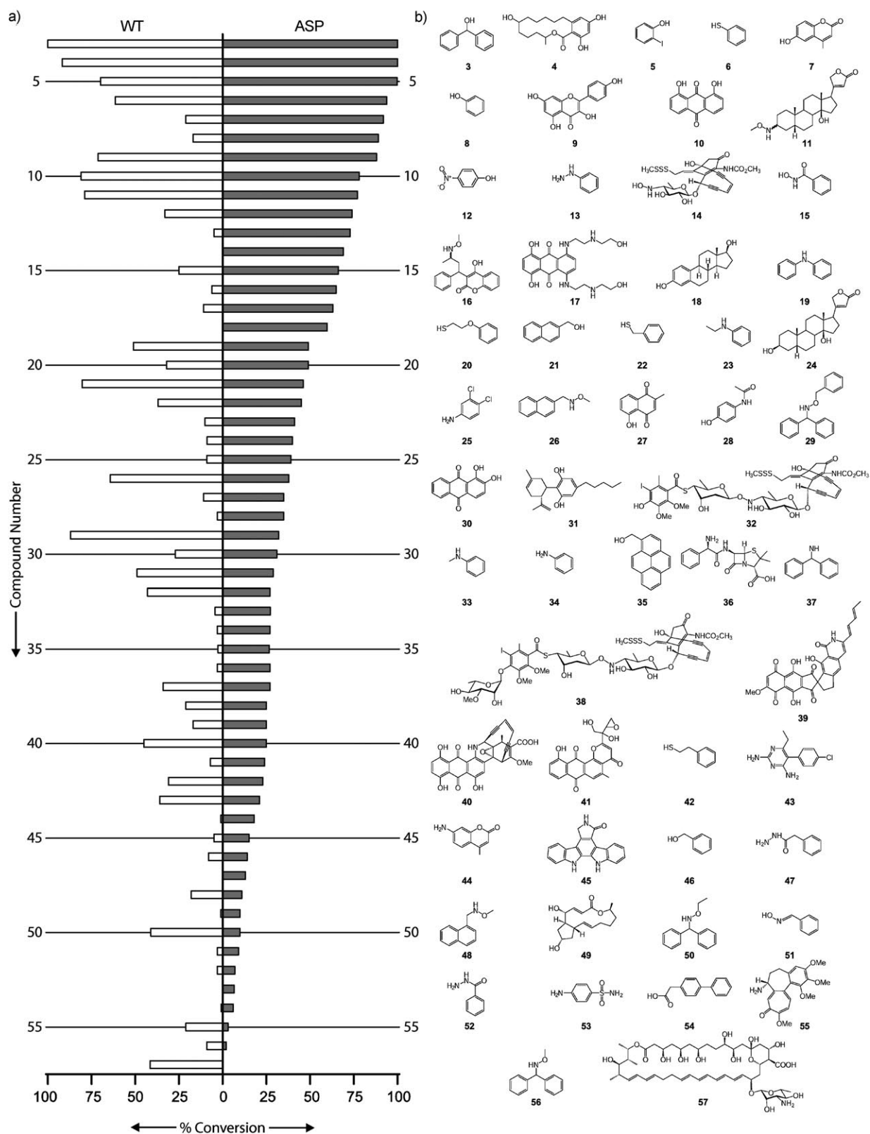
Figure 1. a) Percent conversion of each library member with both WT and ASP OleD. Members are listed in descending order of ASP conversion with numbering corresponding to the structures listed in (b). b) Structures of the corresponding library members. Compounds leading to trace products ( 58–73 , > 5% conversion) or no conversion ( 74–139 ) are listed in the Supporting Information.
